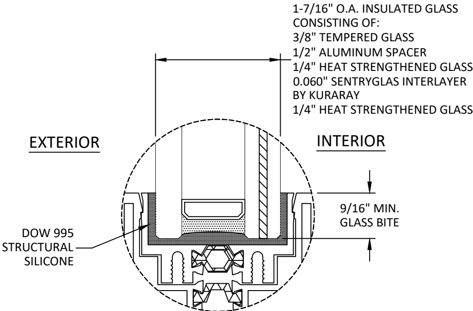
GLAZING DETAIL 1
