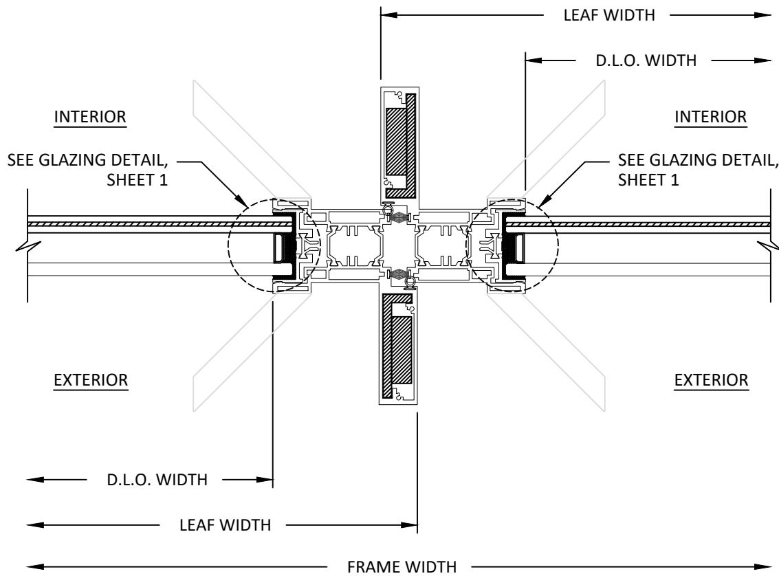
B 8 VERTICAL SECTION MEETING STILE
