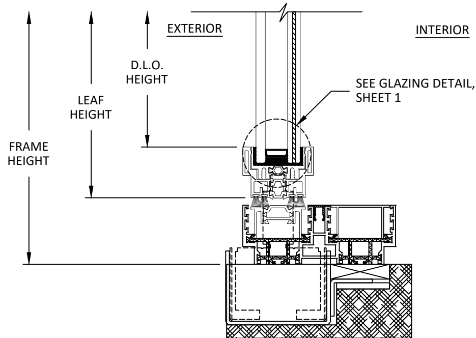
A 7 VERTICAL SECTION PIVOT DOOR SILL
