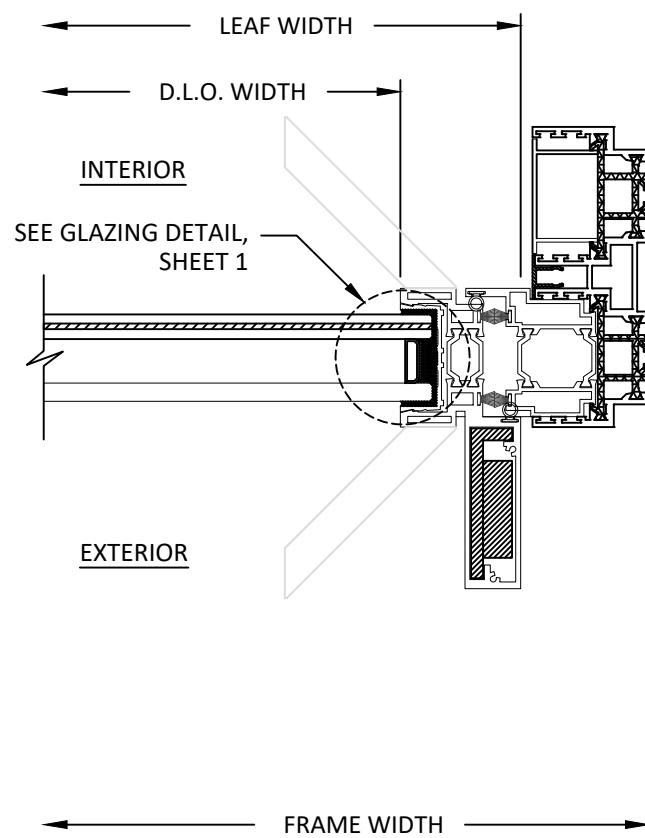
C 8 VERTICAL SECTION LOCK JAMB
