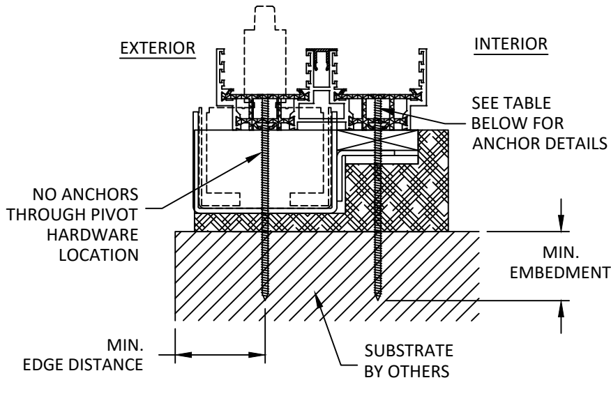
B 9 VERTICAL SECTION SILL - THROUGH FRAME
