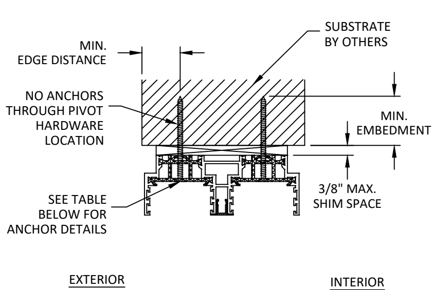
A 9 VERTICAL SECTION HEAD - THROUGH FRAME
