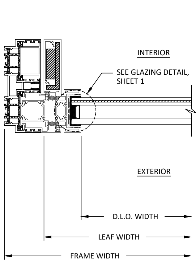
A 8 VERTICAL SECTION JAMB
