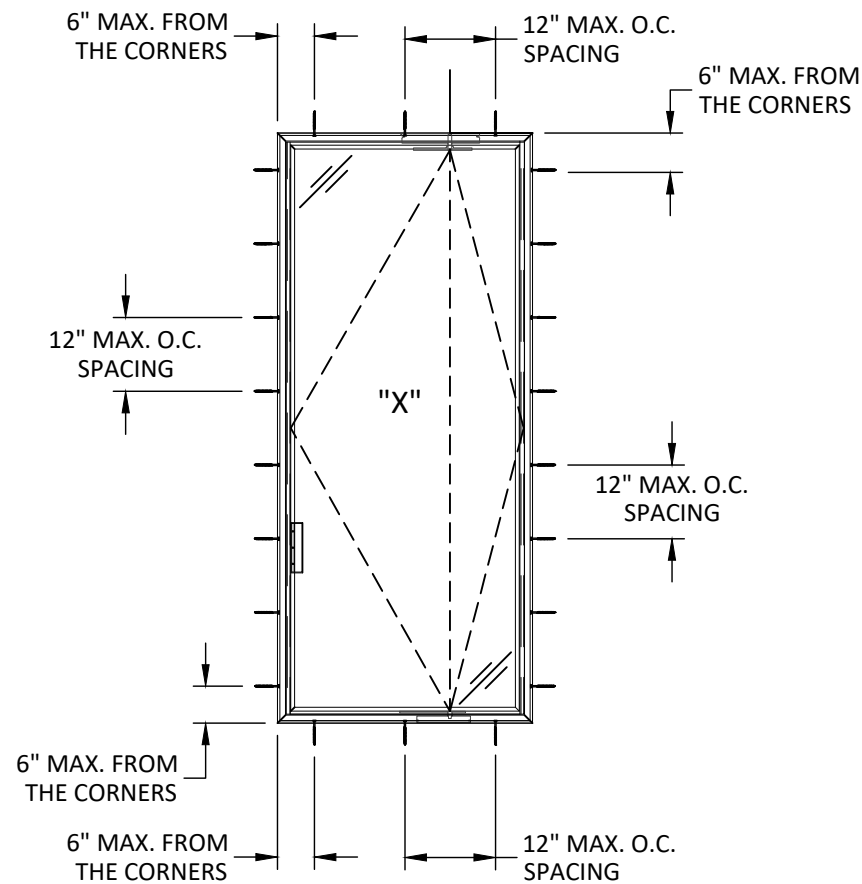
"X" ANCHOR LAYOUT THROUGH FRAME INSTALLATION
